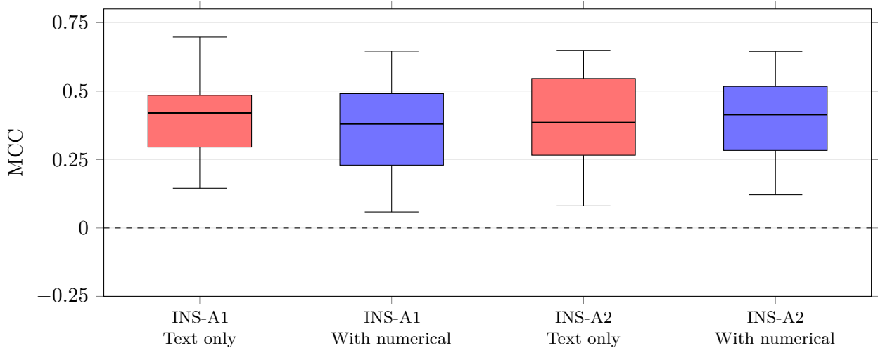
Figure 3: Insufficiency: distribution of MCC across 25 full-depth ( \leq 100 ) case-grouped validation splits. Boxes show the interquartile range, horizontal lines show medians, and whiskers show the observed minimum and maximum.
