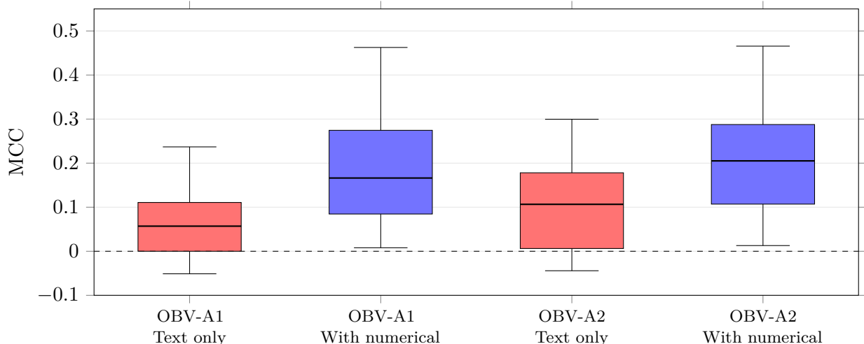
Figure 5: Obviousness: distribution of MCC across 50 full-depth ( \leq 100 ) case-grouped validation splits. Boxes show the interquartile range, horizontal lines show medians, and whiskers show the observed minimum and maximum.
