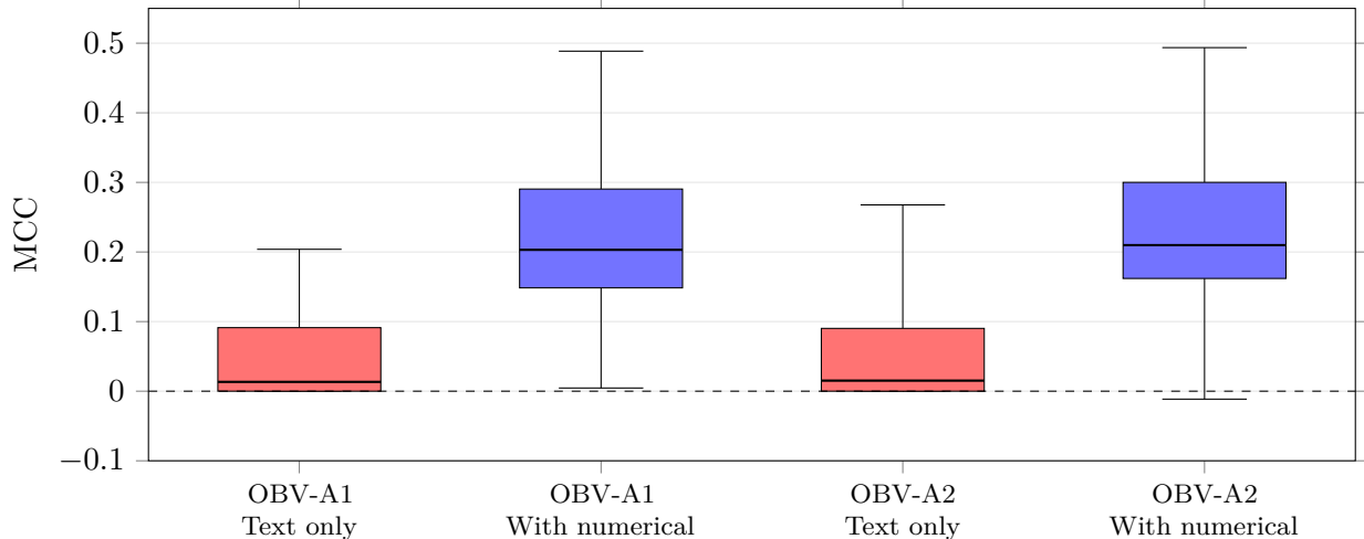
Figure 4: Obviousness: distribution of MCC across 50 depth- \leq 2 case-grouped validation splits. Boxes show the interquartile range, horizontal lines show medians, and whiskers show the observed minimum and maximum.
