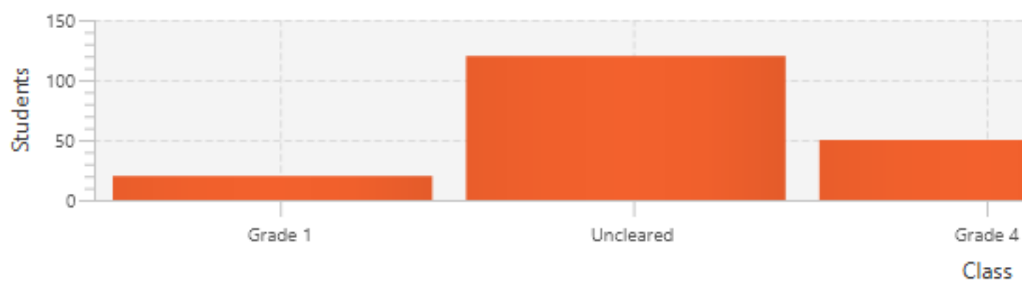
Class Distribution
