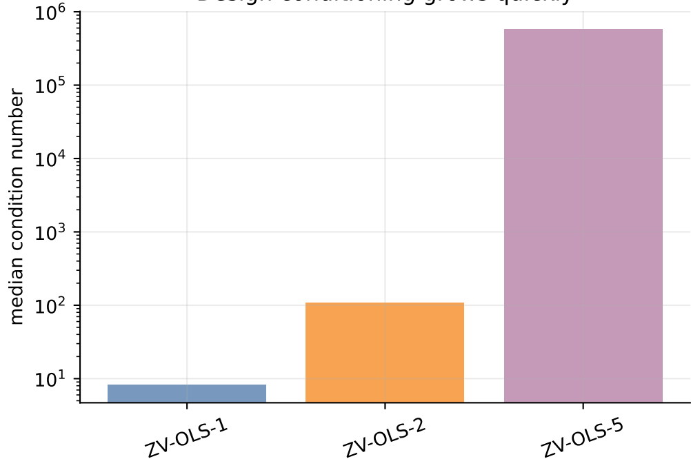
Design conditioning grows quickly
