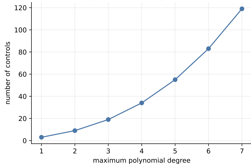
Polynomial dictionary size, d=3
