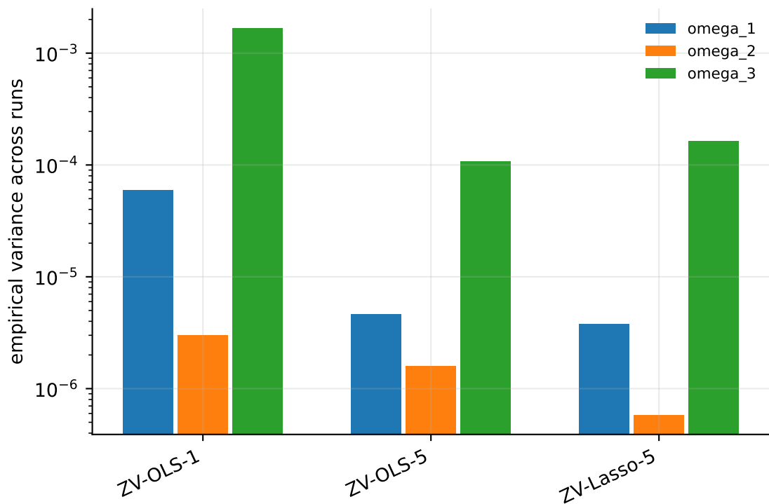
Step 3 variance comparison: large dictionary vs Lasso
