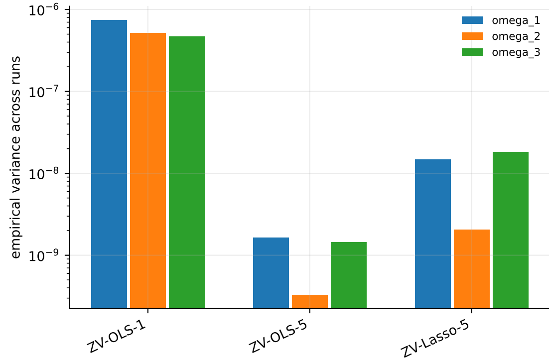
Step 3 variance comparison: large dictionary vs Lasso
