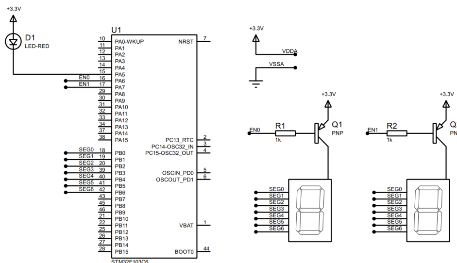
Figure 1.5: Simulation schematic in Proteus
