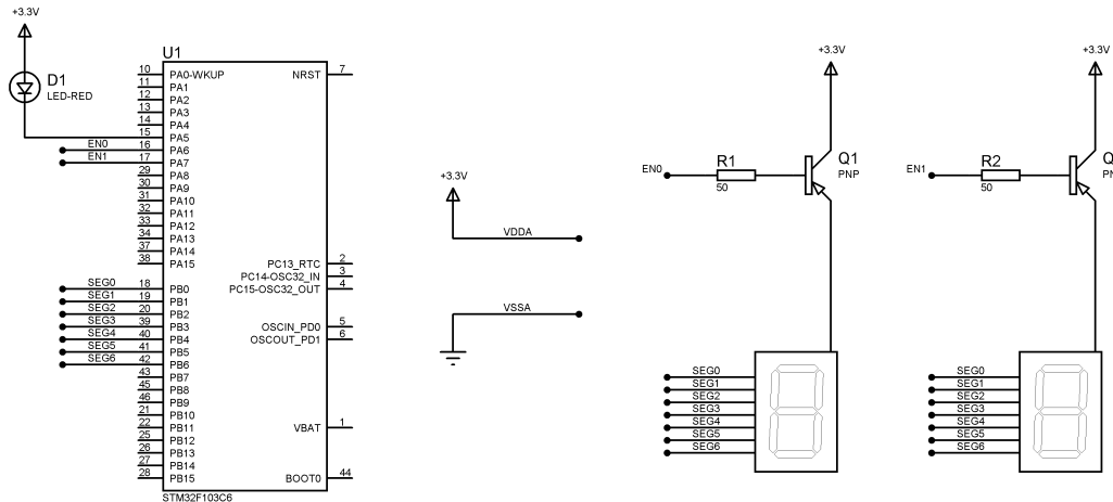
Figure 1.6: Schematic for Exercise 1
