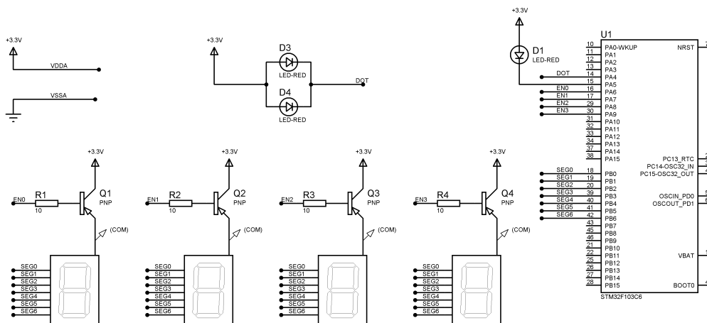
Figure 1.8: Schematic for Exercise 2
