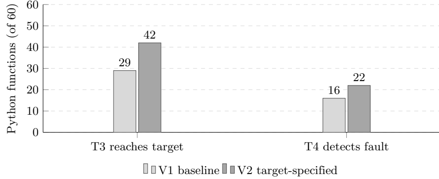
Fig. 1. The split between the two tiers on Python. Adding the target specification lifts the number of suites that reach the target (T3) from 29/60 to 42/60, a significant change, but the number that detects a fault (T4) rises only from 16/60 to 22/60, which is not significant. The prompt improves arrival, not discrimination.
