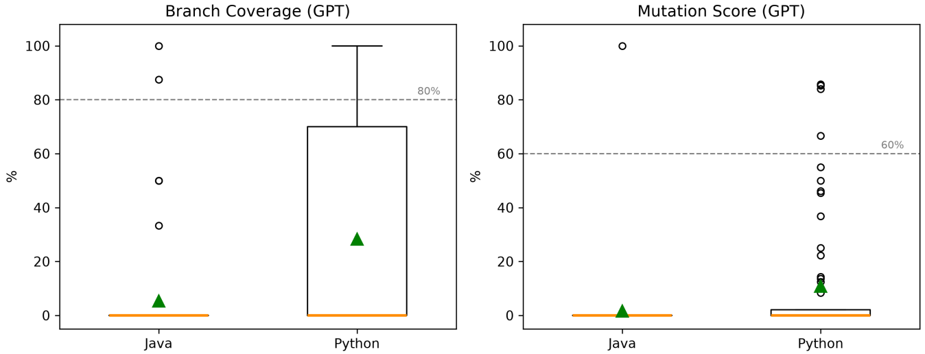
Fig. 2. Branch coverage (left) and mutation score (right) of gpt-4o-mini across all 60 functions per language ( N = 120 ); the median is 0% in every panel (dashed: 80% / 60% thresholds). Effective-subset medians (75.0% Python / 50.0% Java coverage; 36.84% Python mutation) are given in the text.
