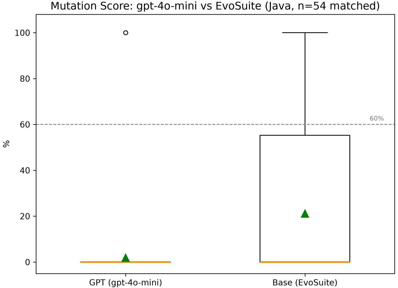
Fig. 2. Mutation score, gpt-4o-mini vs. EvoSuite, matched by function ( n = 54 paired Java functions). EvoSuite wins in every pair where the two differ ( r = -1.00 , p = 0.00044 ).
