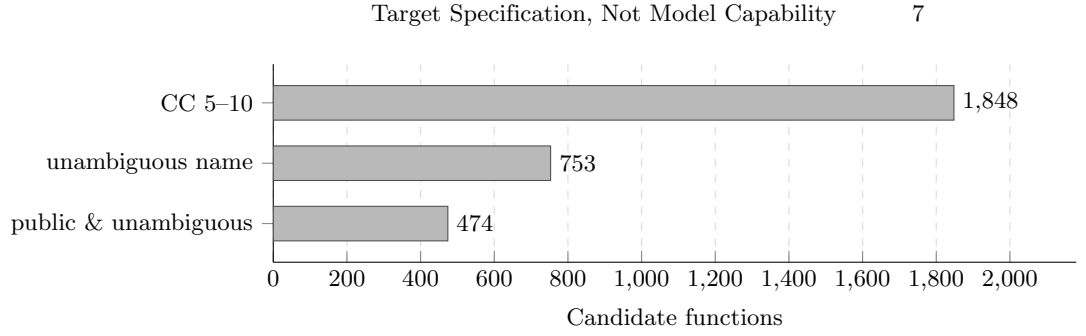
Fig. 1. Attrition of the sampling funnel. Of the 1848 functions in the complexity band, 753 survive the unambiguous-name criterion and 474 are also public — about a quarter of where we started. The remaining three quarters cannot be addressed by an external test at all.
