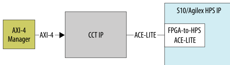
Figure 179. Cache Coherency Translator (CCT) Use Case
