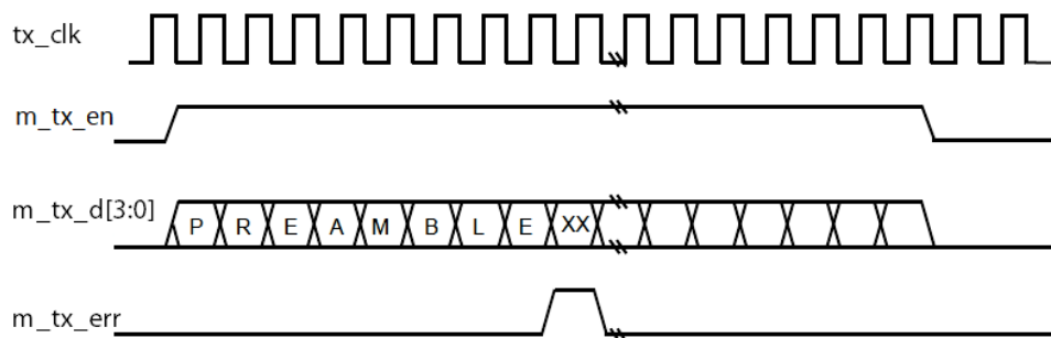
Figure 168. TX Frame with Error Signal
