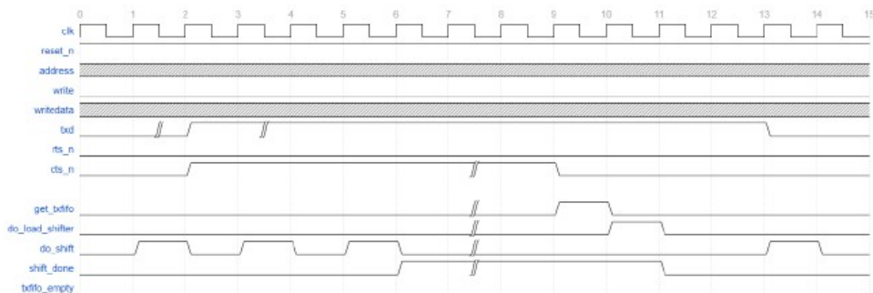
Figure 187. Flow Control in Lightweight UART Transmitter
