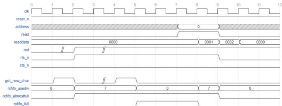
Figure 188. Flow Control in Lightweight UART Receiver
