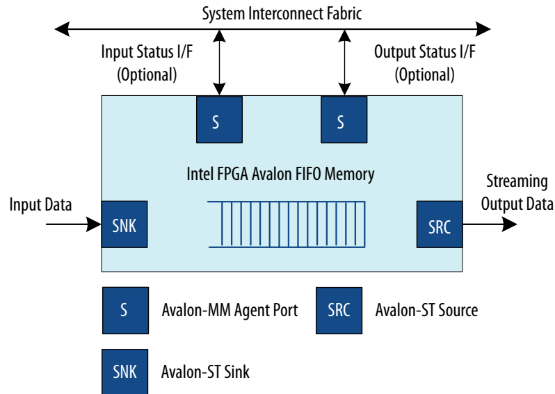
Figure 75. FIFO with Avalon-ST Input and Output Interfaces
