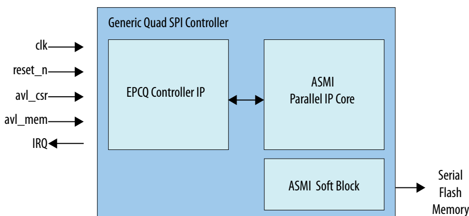
Figure 70. Intel FPGA Generic QUAD SPI Controller Block Diagram
