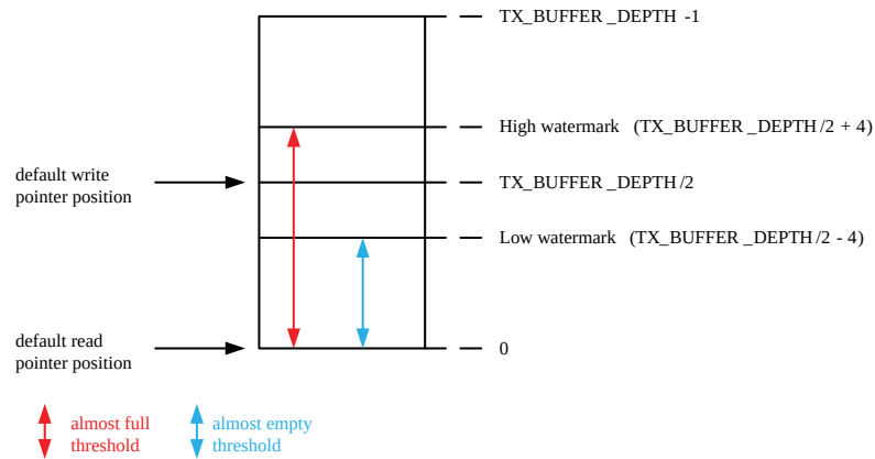
Figure 173. Elastic Buffer Watermark Level
