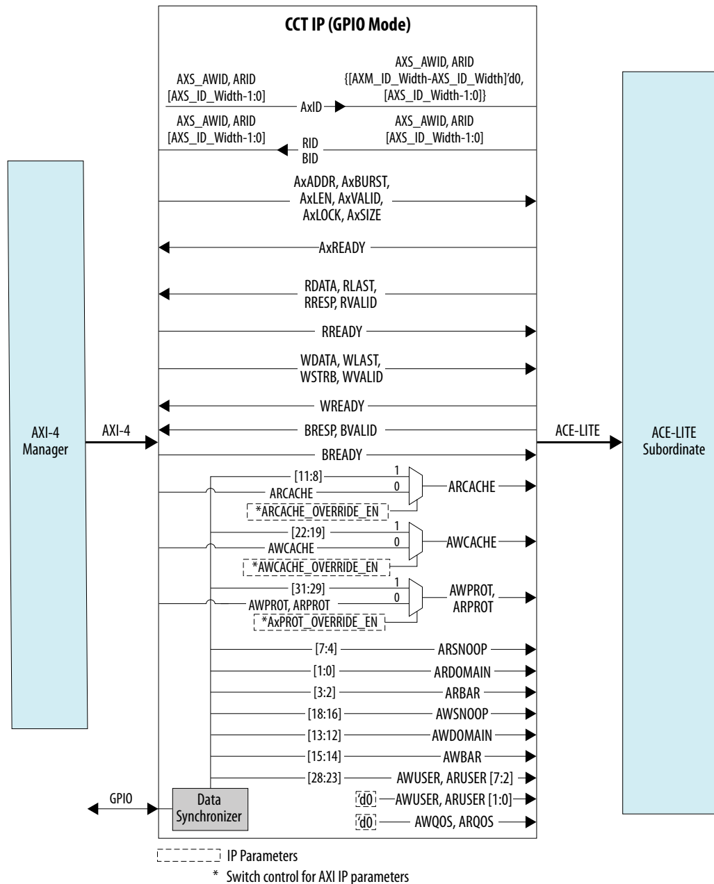
Figure 184. Block Diagram for GPIO Mode
