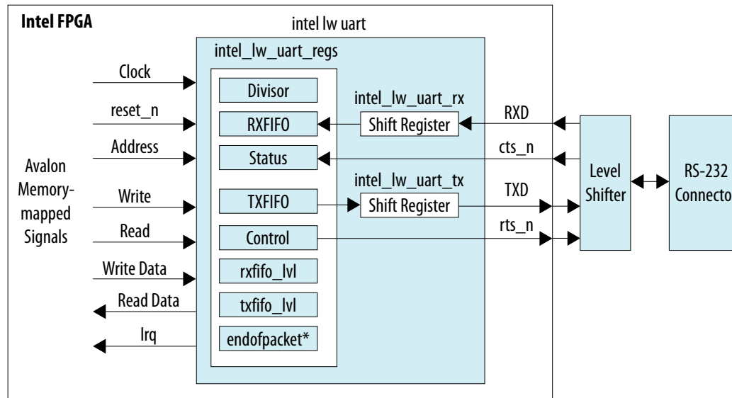
Figure 186. Block Diagram of Lightweight UART Core in a Typical System
