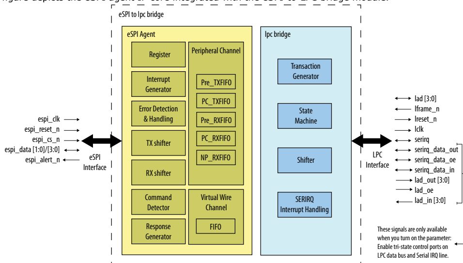
Figure 27. Block Diagram
