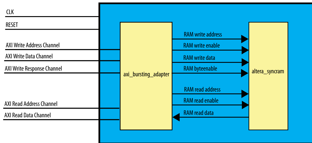
Figure 82. Block Diagram with AXI Interface
