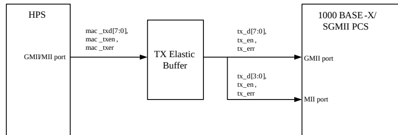
Figure 171. Transmit Data Path
