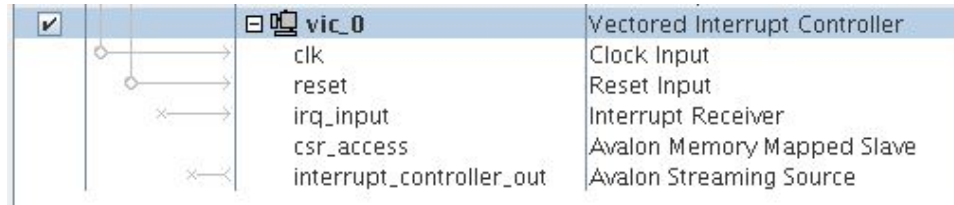
Figure 140. VIC Interfaces
