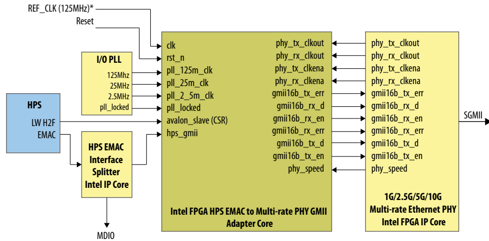
Figure 175. Block Diagram
