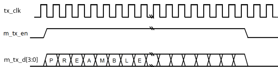
Figure 167. MII TX Frame
