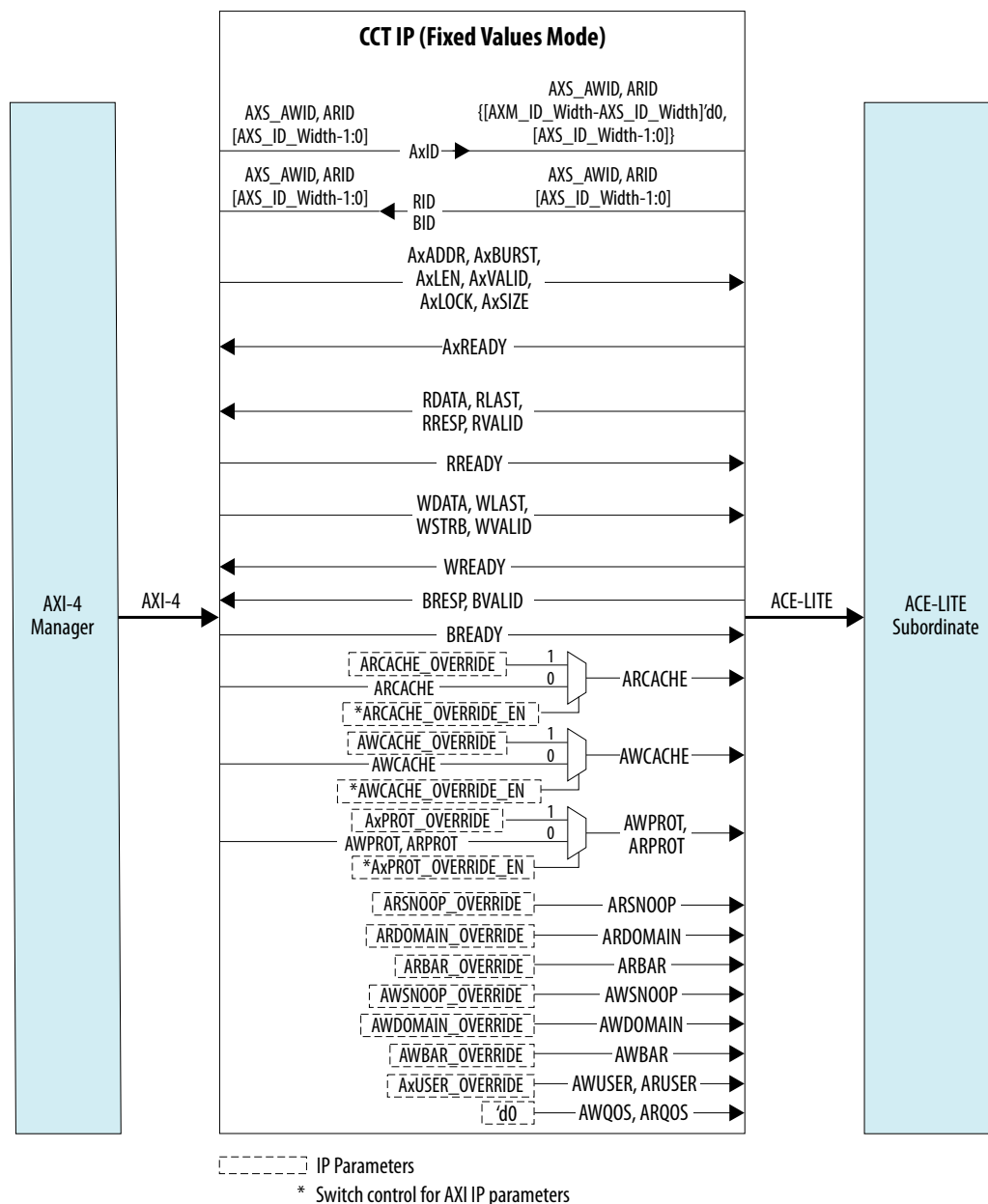
Figure 183. Block Diagram for Fixed Value Mode
