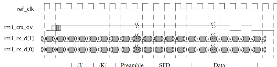
Figure 169. RMII Receive Transfer
