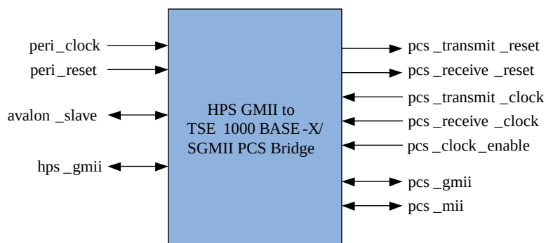
Figure 174. HPS GMII to TSE 1000BASE-X/SGMII PCS Bridge Intel FPGA IP Top Level Interfaces
