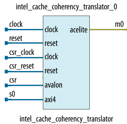
Figure 182. CSR Mode Block Diagram (CONTROL_INTERFACE = 2 (CSR))
