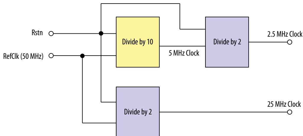
Figure 166. Clocking Scheme
