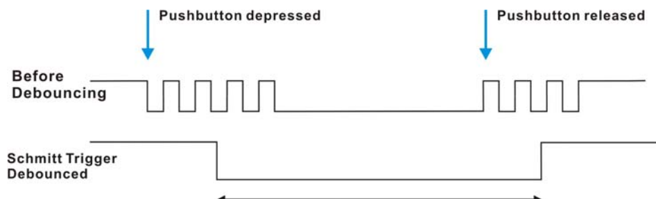
Figure 4.3. Switch debouncing.
