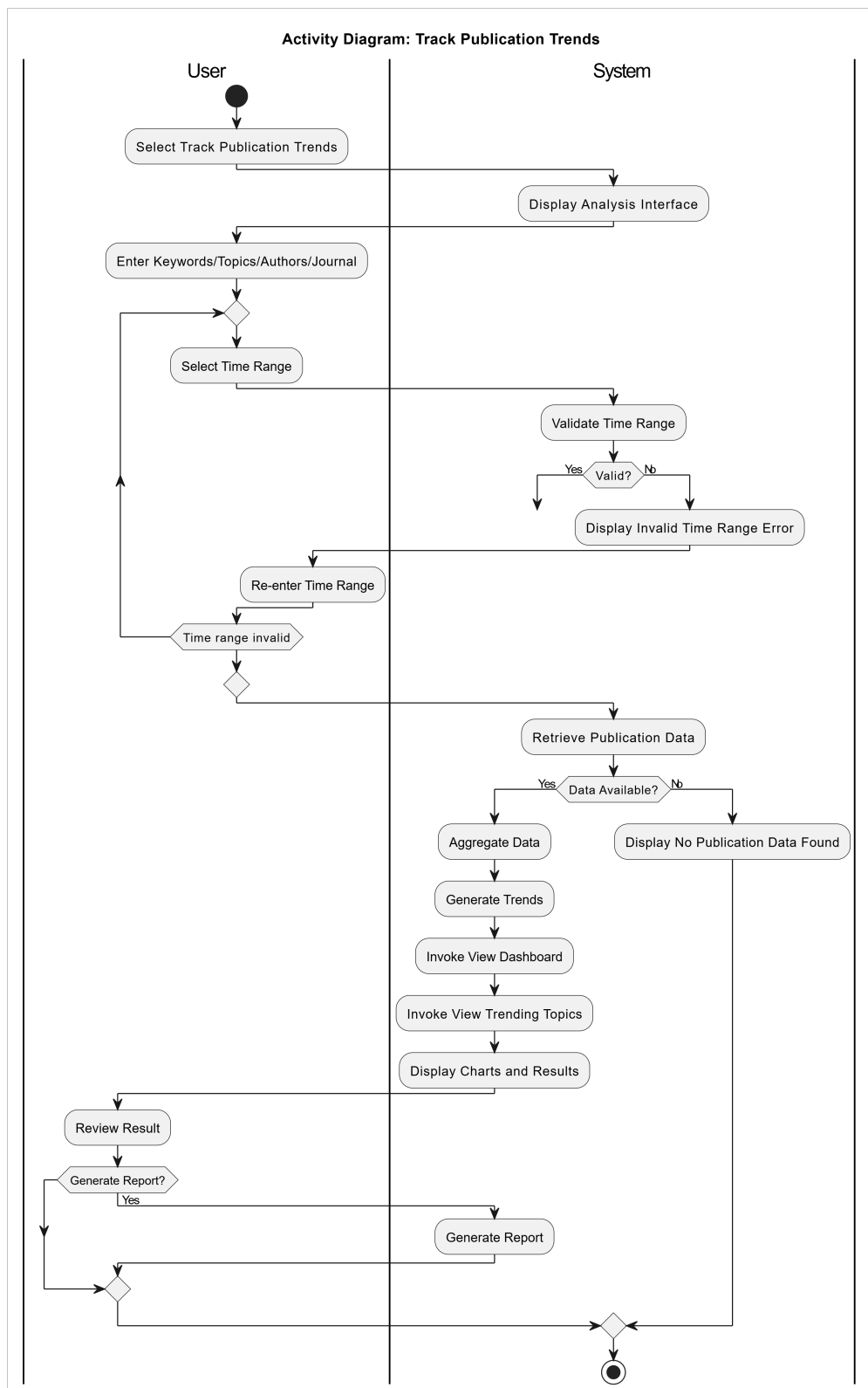
Hình 35: Activity Diagram: Track Publication Trends
