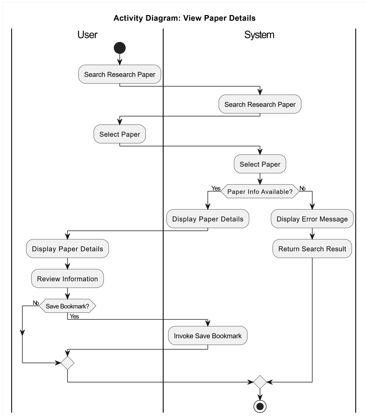
Hình 55: Activity Diagram: View Paper Details
