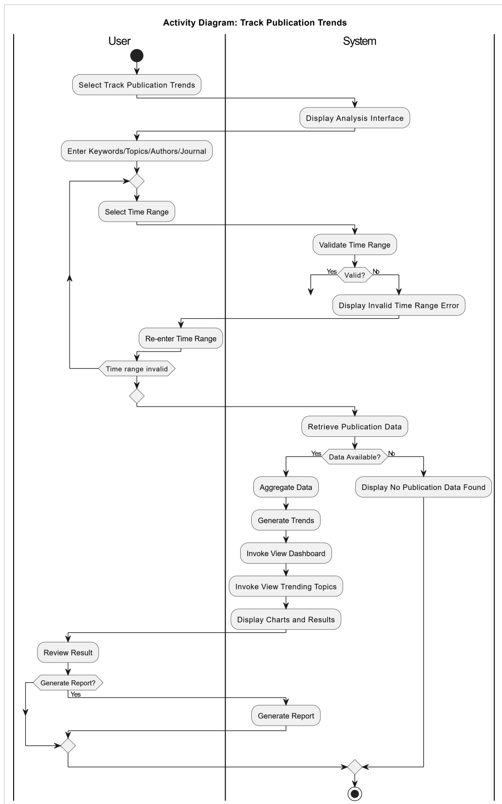
Hình 63: Activity Diagram: Track Publication Trends
