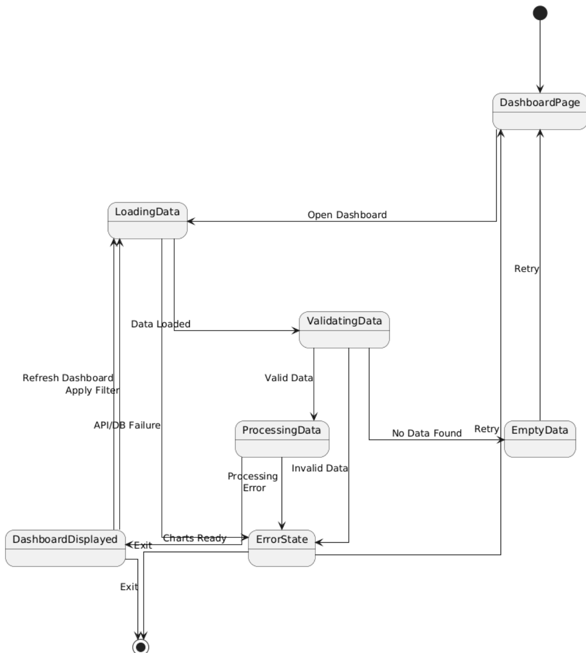
State Diagram - View Dashboard
