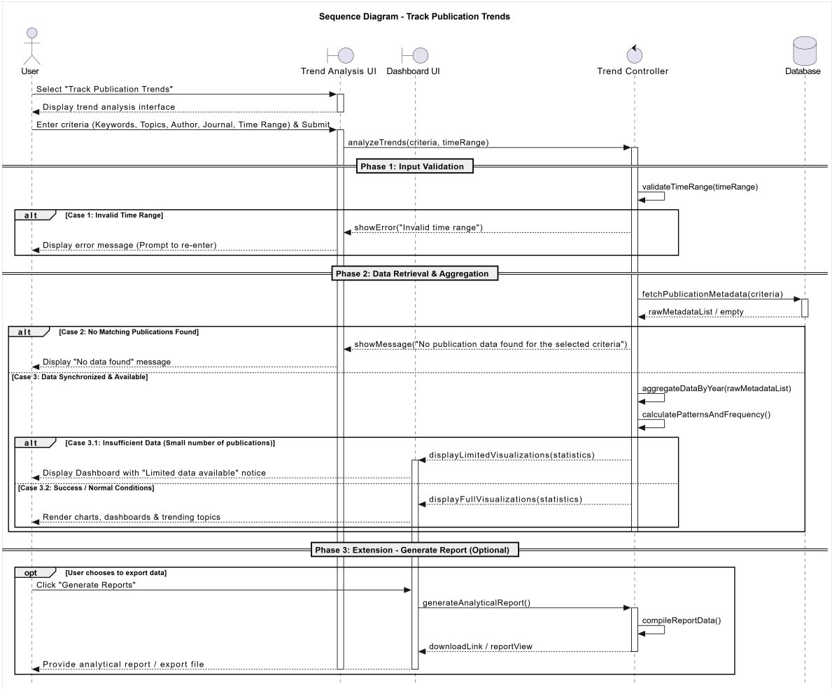
Hình 32: Sequence Diagram: Track Publication Trends
