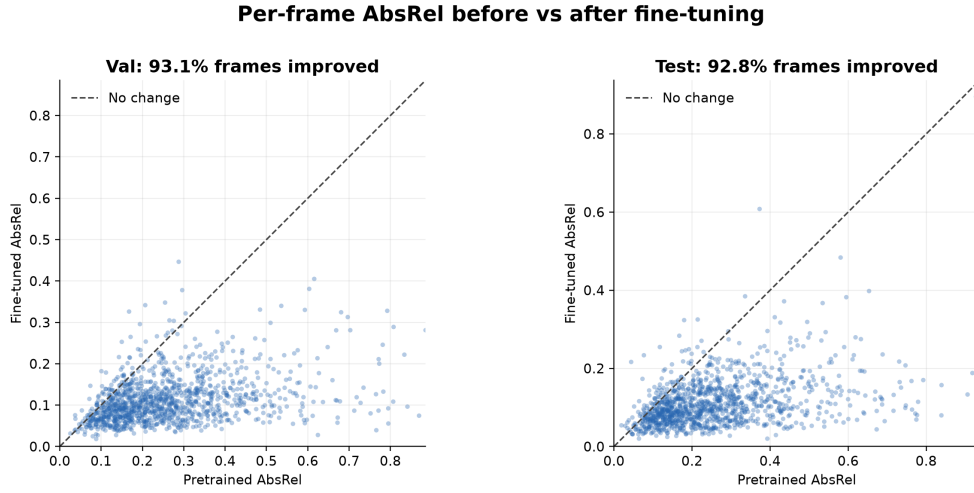
(b) AbsRel scatter before and after fine-tuning.
