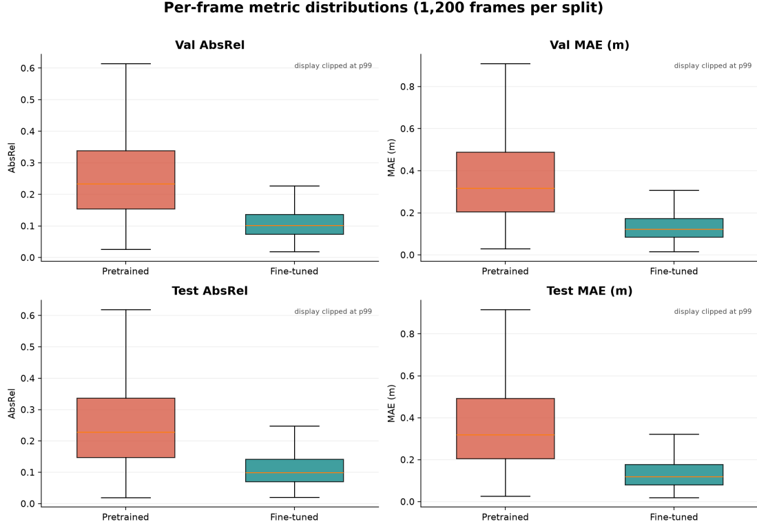
(a) Per-frame distributions of depth metrics.
