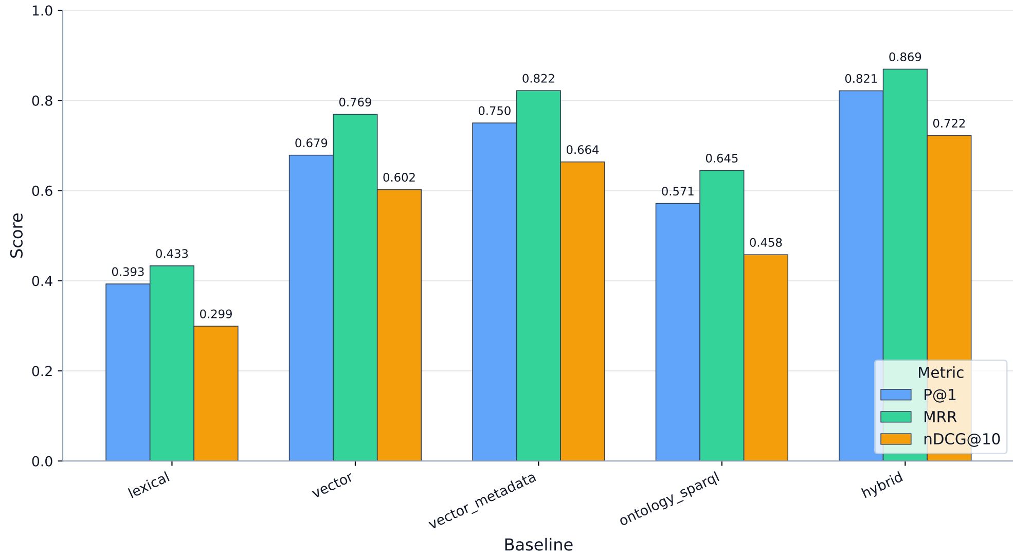
Key retrieval metrics by baseline
