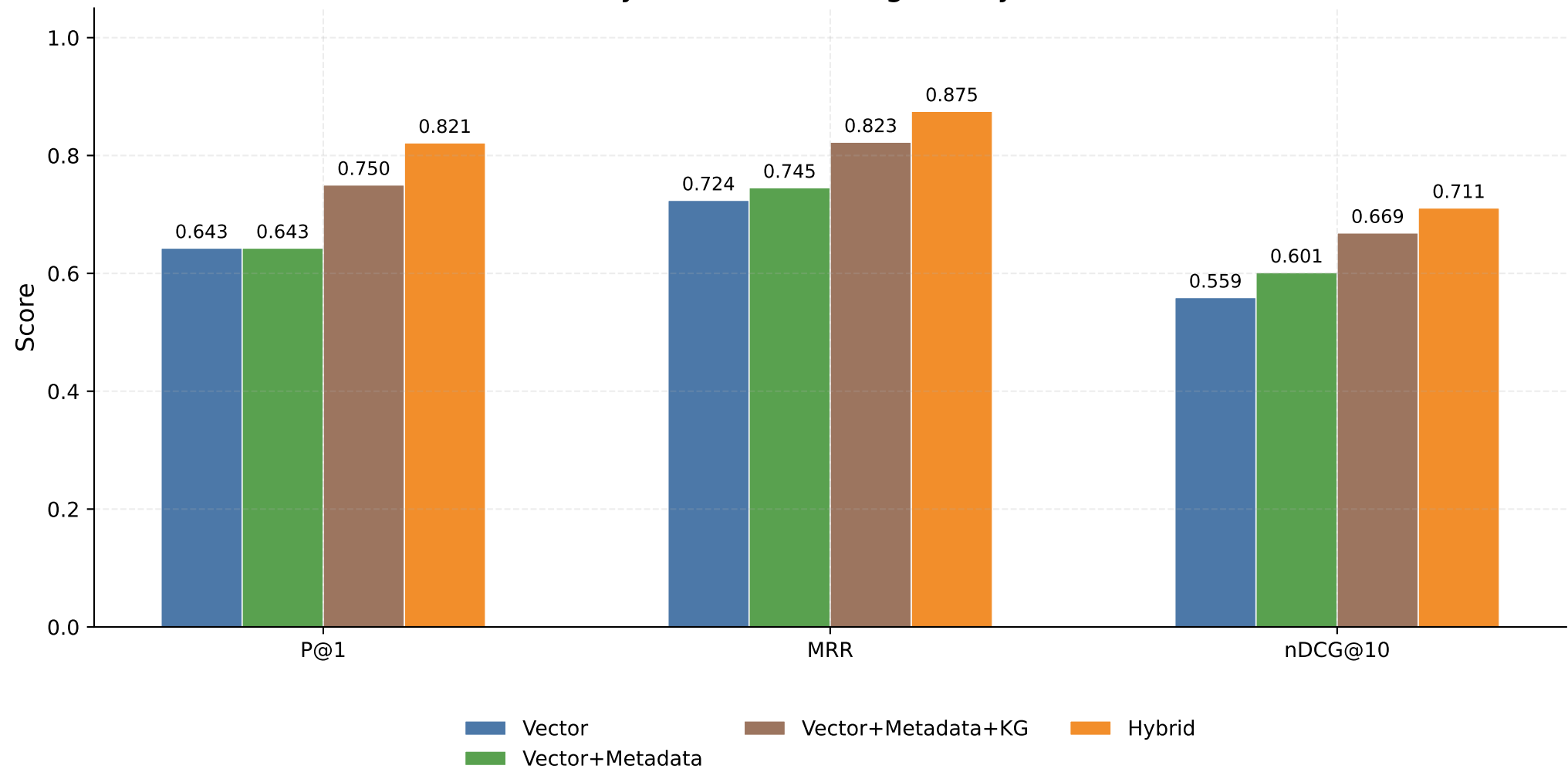
Hybrid Ablation: Signal Layers
