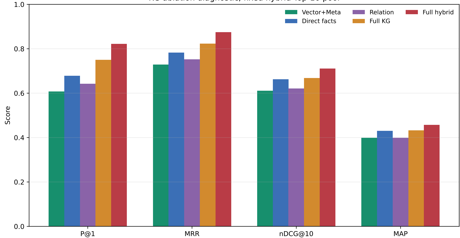
KG ablation diagnostic, fixed hybrid Top-10 pool
