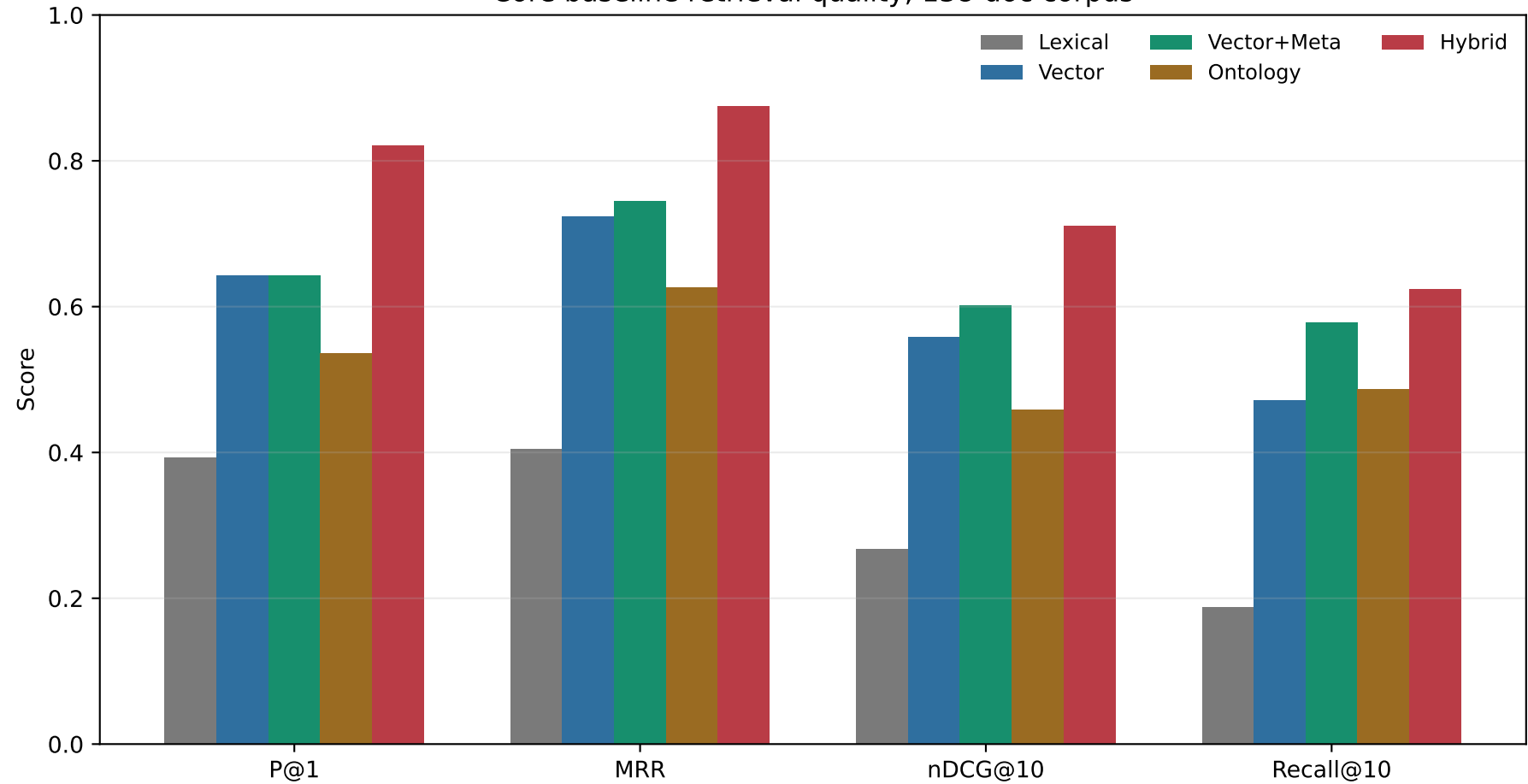
Core baseline retrieval quality, 138-doc corpus
