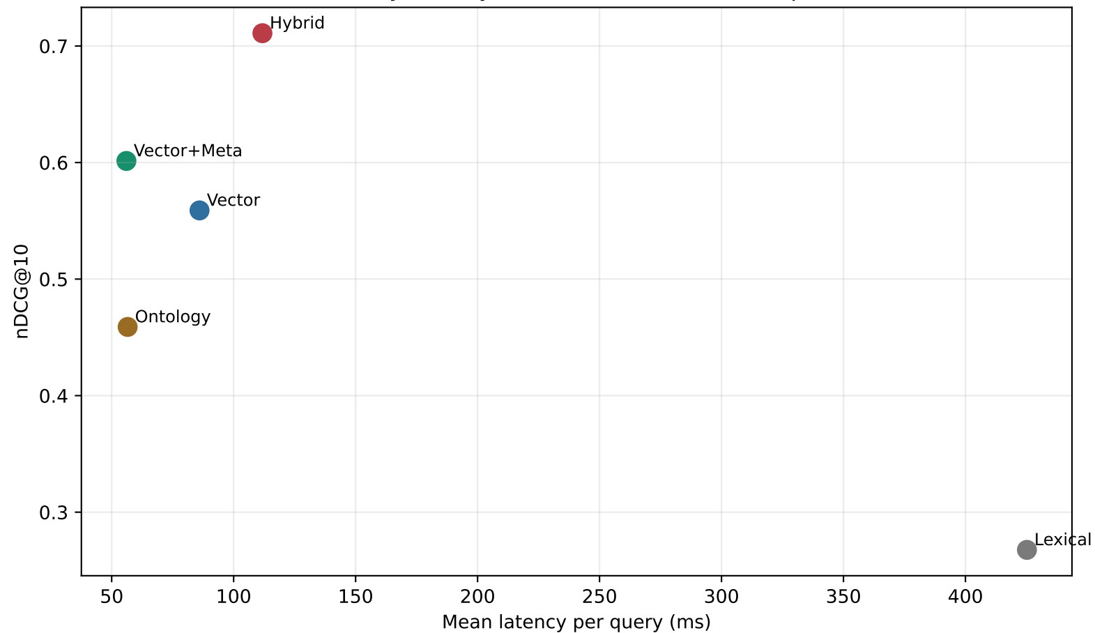
Quality-latency tradeoff, core 138-doc corpus
