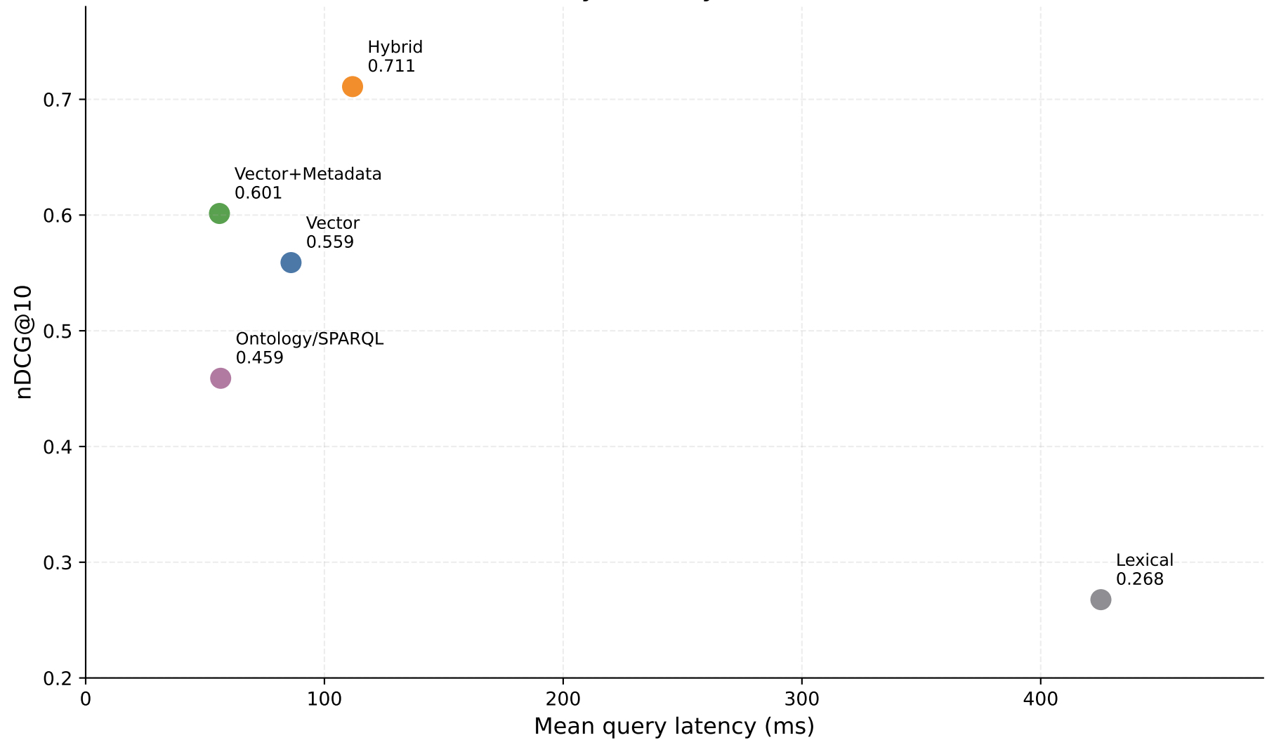
Quality-Latency Trade-off
