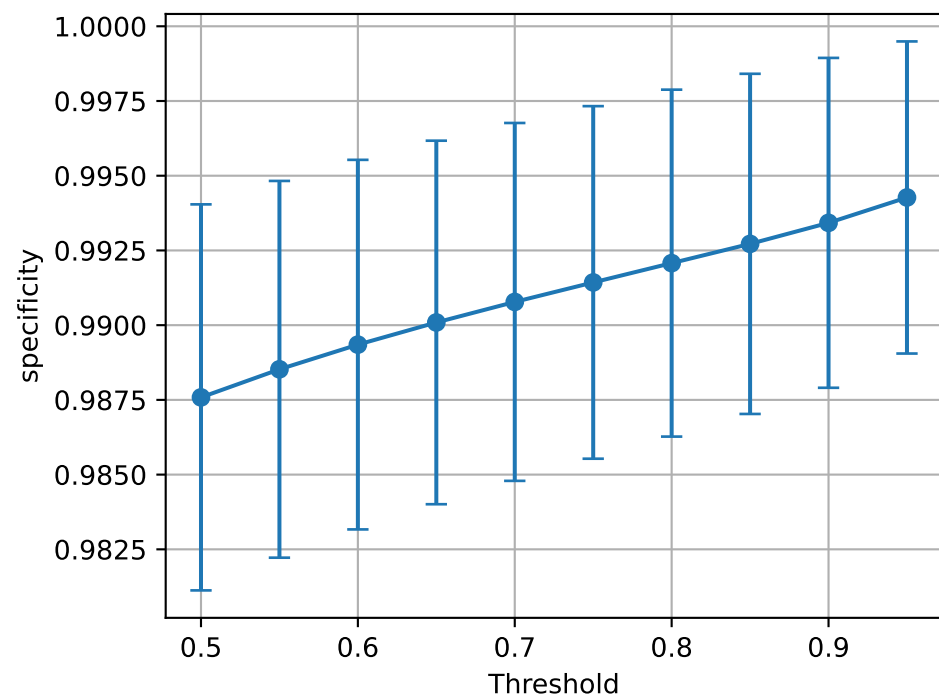
SPECIFICITY
