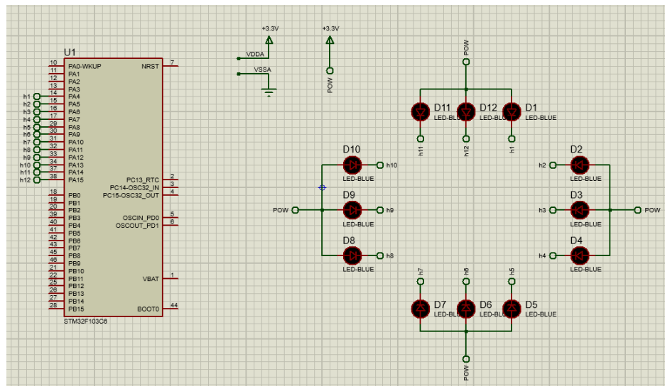
Hình 1.32: Proteus Schematic for Exercise 6. The source code and project files can be accessed at: GitHub Repository
