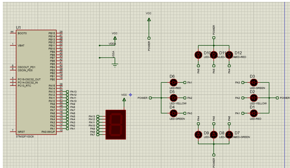
Hình 1.30: Proteus Schematic for Exercise 5. The source code and project files can be accessed at: GitHub Repository
