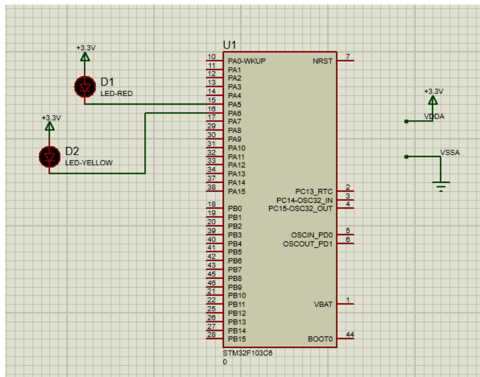
Hình 1.24: Proteus Schematic for Exercise 1. The source code and project files can be accessed at: GitHub Repository
