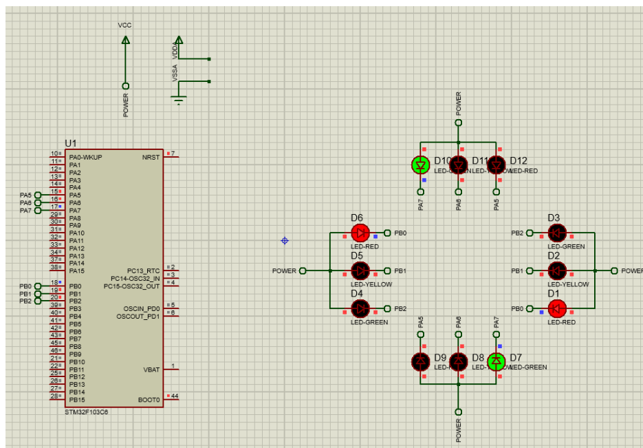
Hình 1.27: Proteus Schematic for Exercise 3. The source code and project files can be accessed at: GitHub Repository
