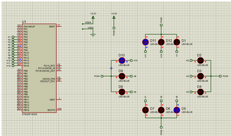
Hình 1.33: Proteus Schematic for Exercise 10. The source code and project files can be accessed at: GitHub Repository
