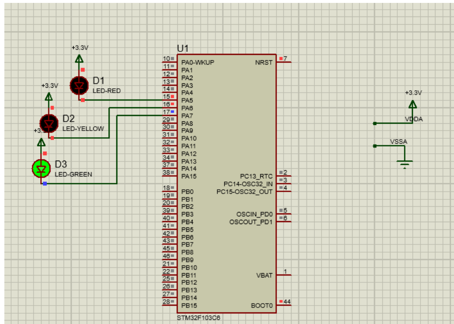
Hình 1.25: Proteus Schematic for Exercise 2. The source code and project files can be accessed at: GitHub Repository
