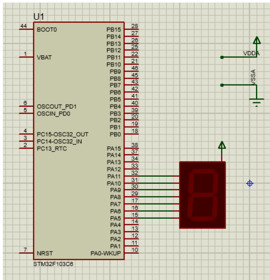
Hình 1.29: Proteus Schematic for Exercise 4. The source code and project files can be accessed at: GitHub Repository
