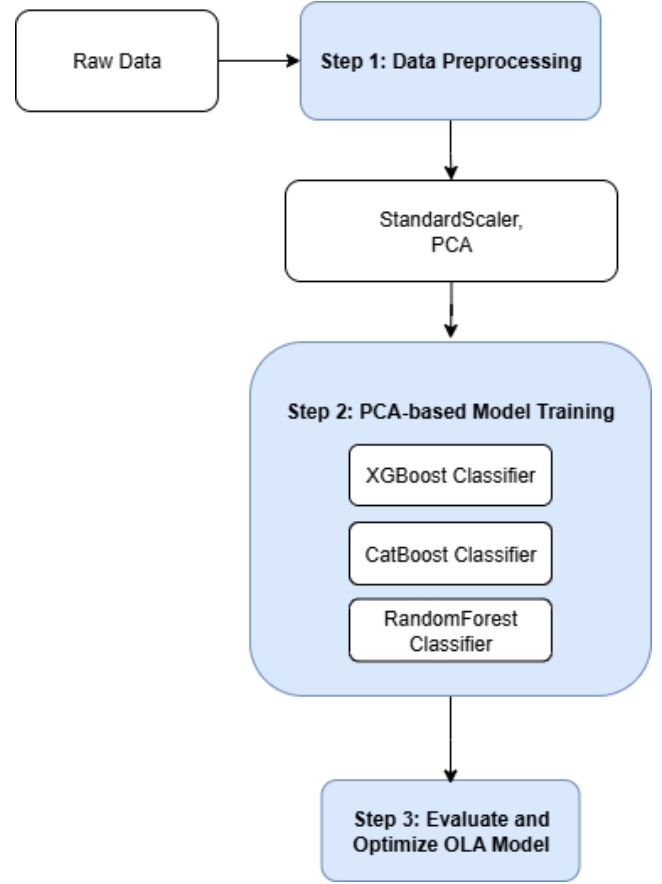
Fig. 2: Framework OLA
