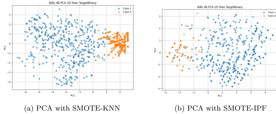
Fig. 3: Comparison of PCA visualizations on private dataset using SMOTE-KNN and SMOTE-IPF.
