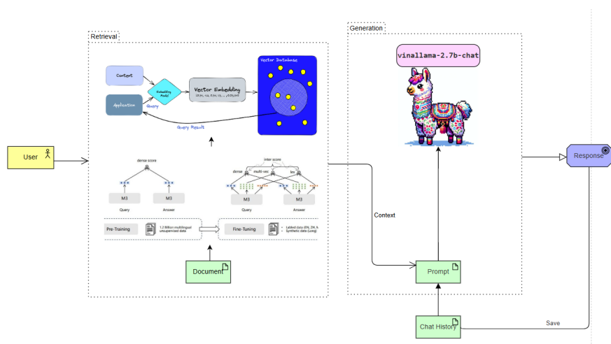
Figure 1: System architecture of the proposed RAG-based consulting assistant using LangChain and vinallama-2.7b-chat.
