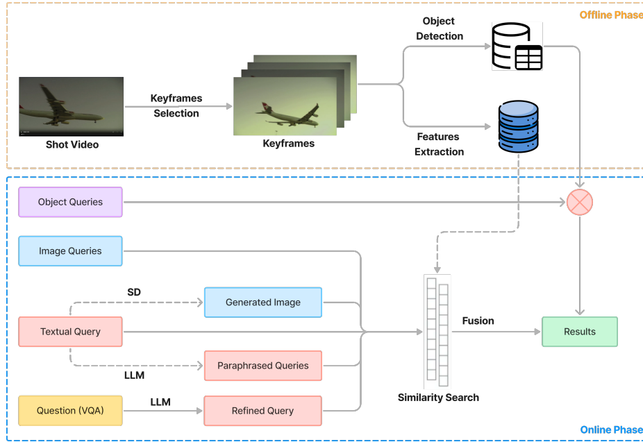
Fig. 1. The proposed system operates in two stages: offline and online. In the offline stage, datasets are processed and indexed for efficient querying. In the online phase, the system analyzes user queries, searches the database, and presents relevant results.
