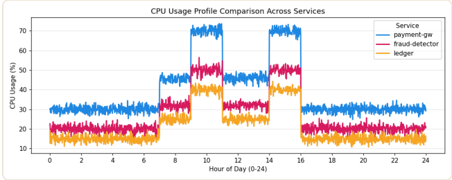
Fig — 3 services exhibiting entirely different daily traffic behaviors. A 1-size-fits-all static threshold is impossible.
