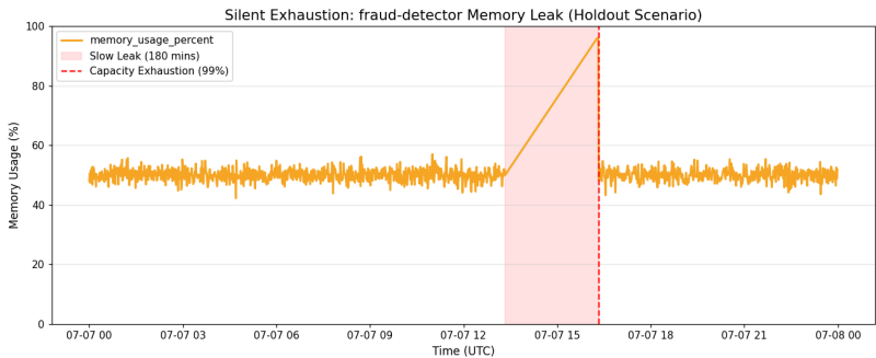
Fig. 2 — A memory leak creeping up silently for 180 minutes. The 99% mark (Static threshold) flashes red only upon crashing. Lead time = 0.
