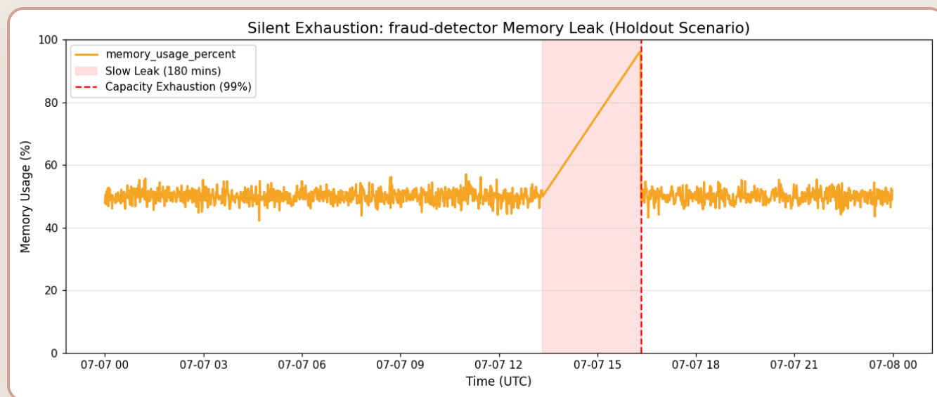
Fig. 2 — A memory leak creeping up silently for 180 minutes. The 99% mark (Static threshold) flashes red only upon crashing. Lead time = 0.
