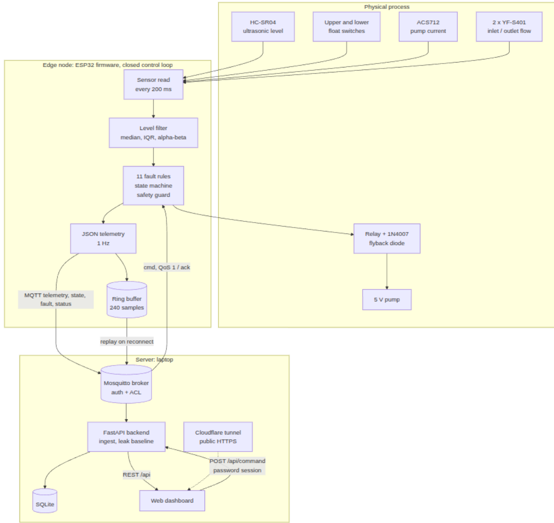
Figure 2.1.1: Architecture of the smart water tank system. The closed control loop lives entirely inside the edge node.
