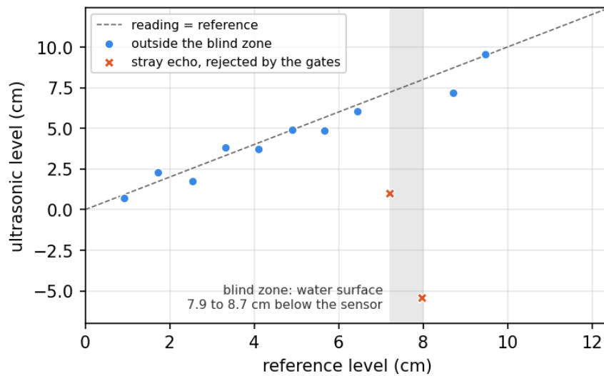
Figure 5.2.1: E1: ultrasonic level against the reference level. Crosses mark the blind zone, where the sensor returns a stray echo instead of the surface.
