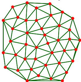
Delaunay
