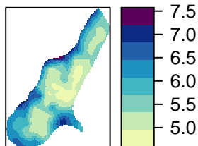
Kriging prediction
