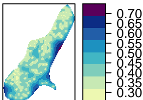
Kriging standard error
