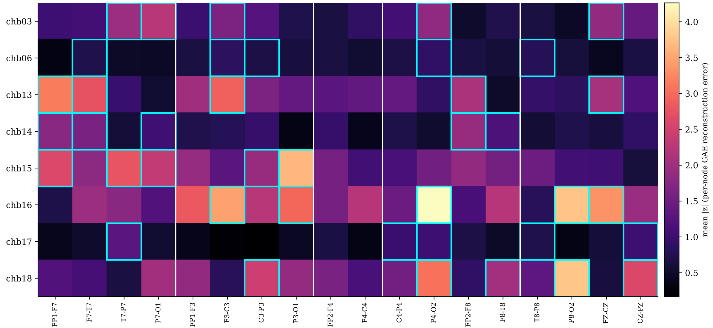
Channel attribution -- per-node GAE reconstruction error (cyan border = top 5 attributed channel for that subject)
