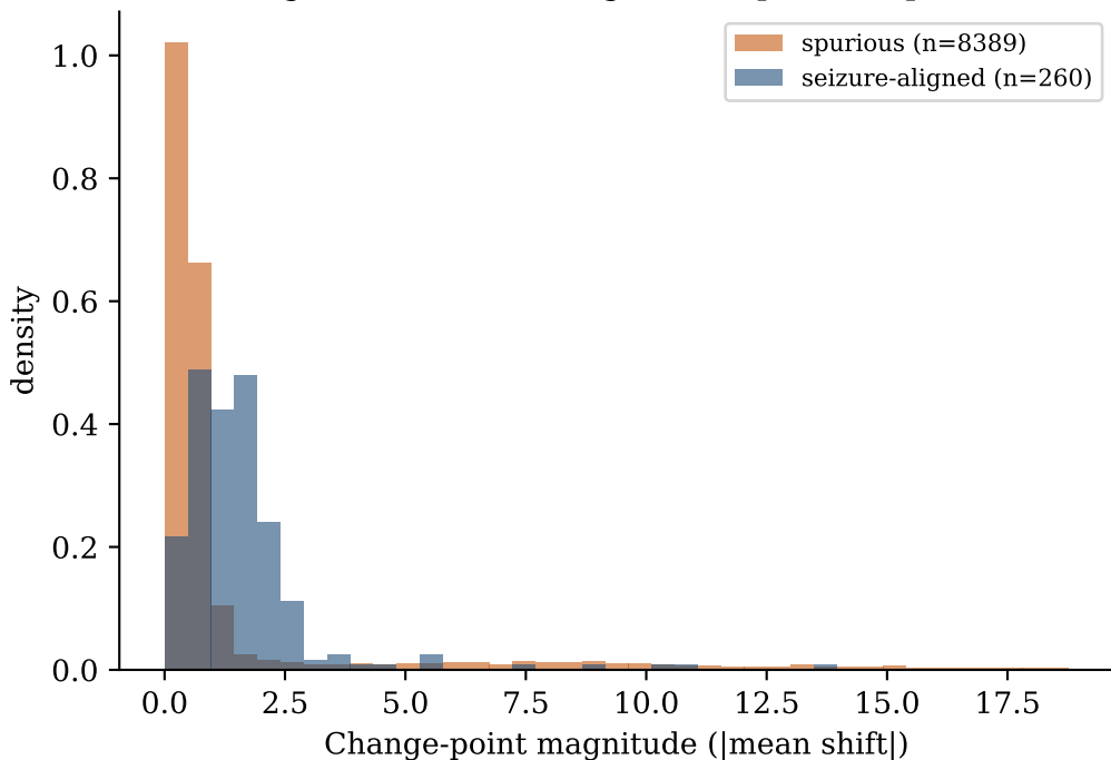
CP magnitude: seizure-aligned vs spurious (pen=0.3)
