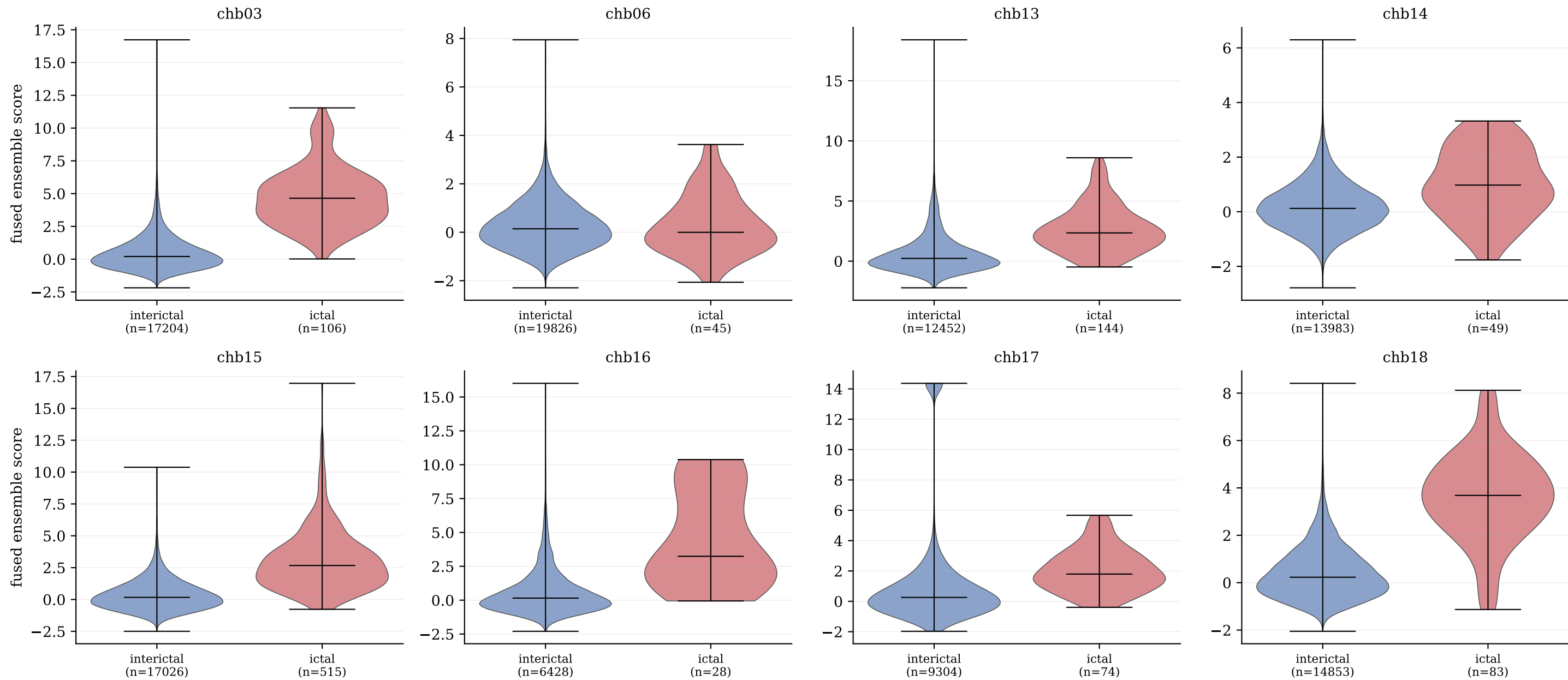
Fig 3.2 — fused ensemble score distributions per patient, held-out set (seed 42, final system)
