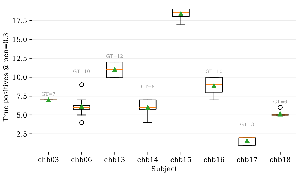
Per-subject TP stability across padding seeds (pen=0.3)
