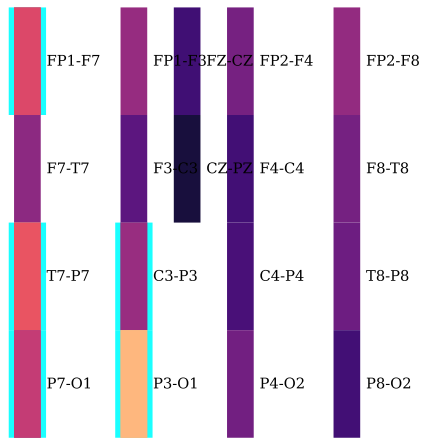
chb15 [CSF] LI=+0.24
