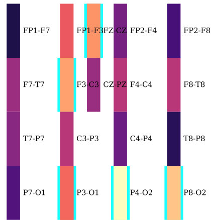
chb16 [CS-] LI=-0.01
