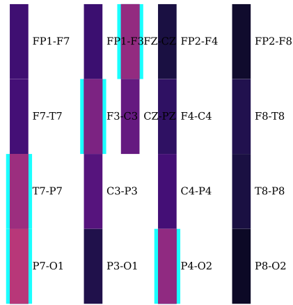
chb03 [CS-] LI=+0.23
