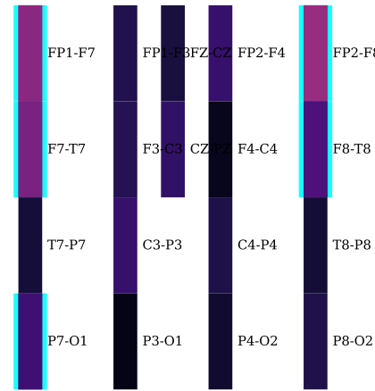
chb14 [CSF] LI=+0.06
