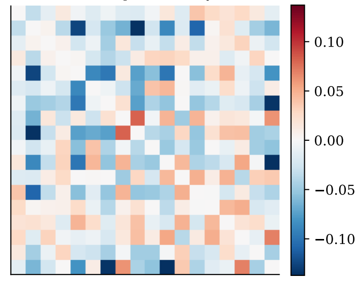
chb06: ictal - inter (predominantly NEGATIVE)
