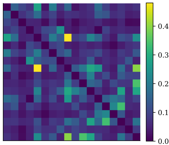
chb18: mean ictal
