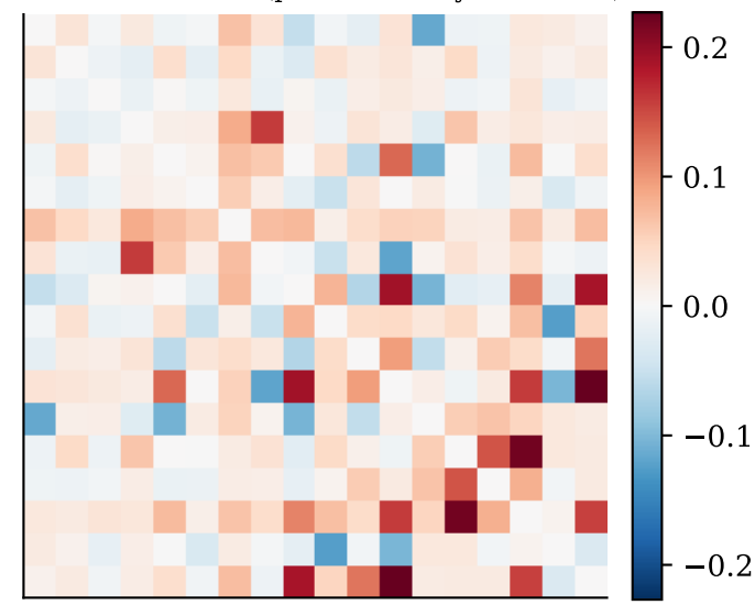
chb18: ictal - inter (predominantly POSITIVE)
