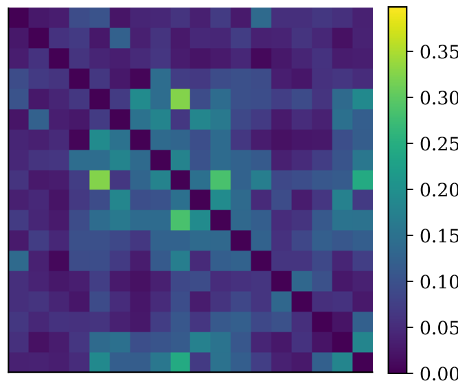
chb06: mean ictal
