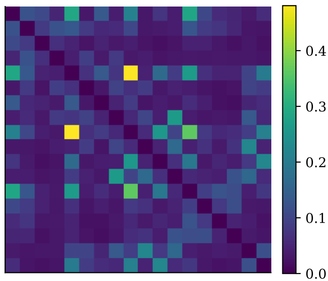
chb18: mean interictal
