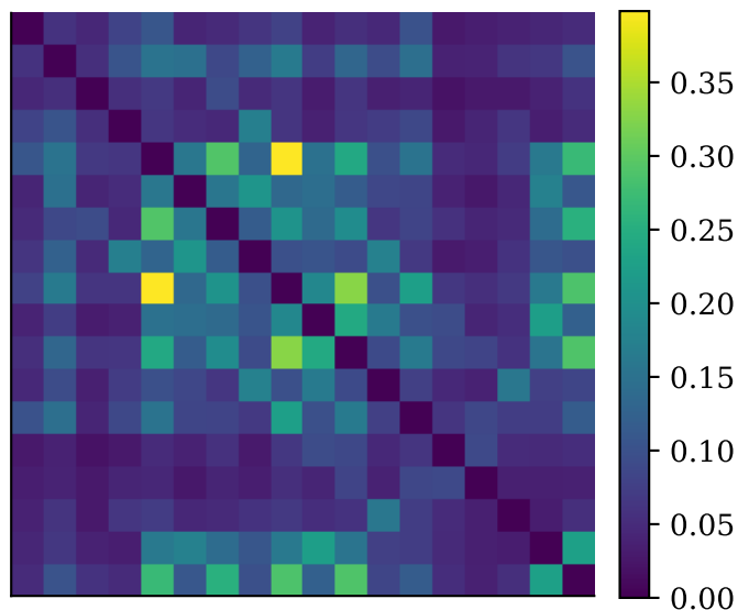
chb06: mean interictal
