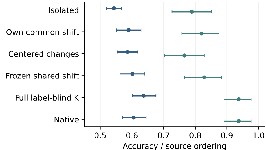
Shared offset restores prediction partially
