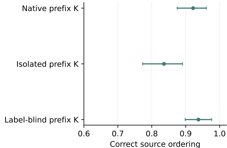
History dependence \neq label-rule content
