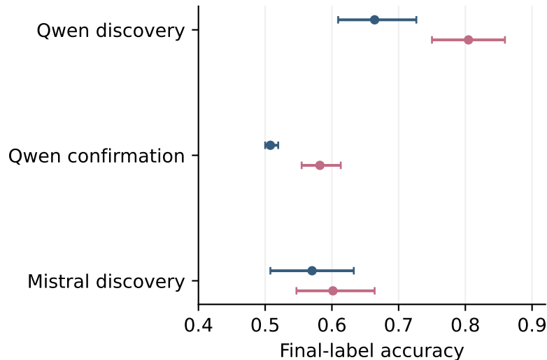
Same final label; encoding matters
