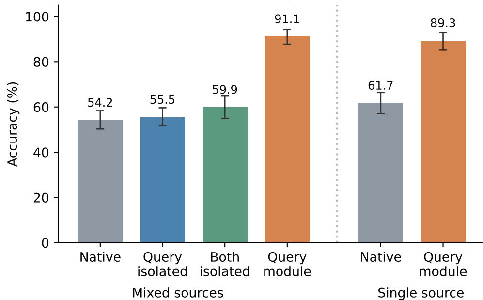
A Source exclusion does not reproduce learned readout 48 new contexts; same frozen query module
