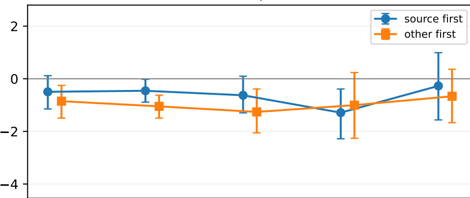
contrast parent
