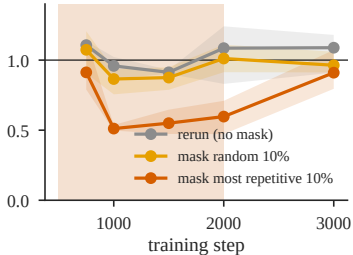
b copying ability
