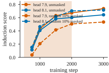
c two candidates (initialization 2)
