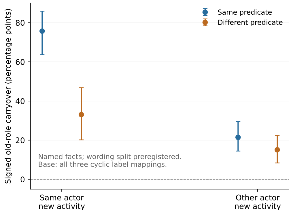
B. Relation classifications retain old direction
