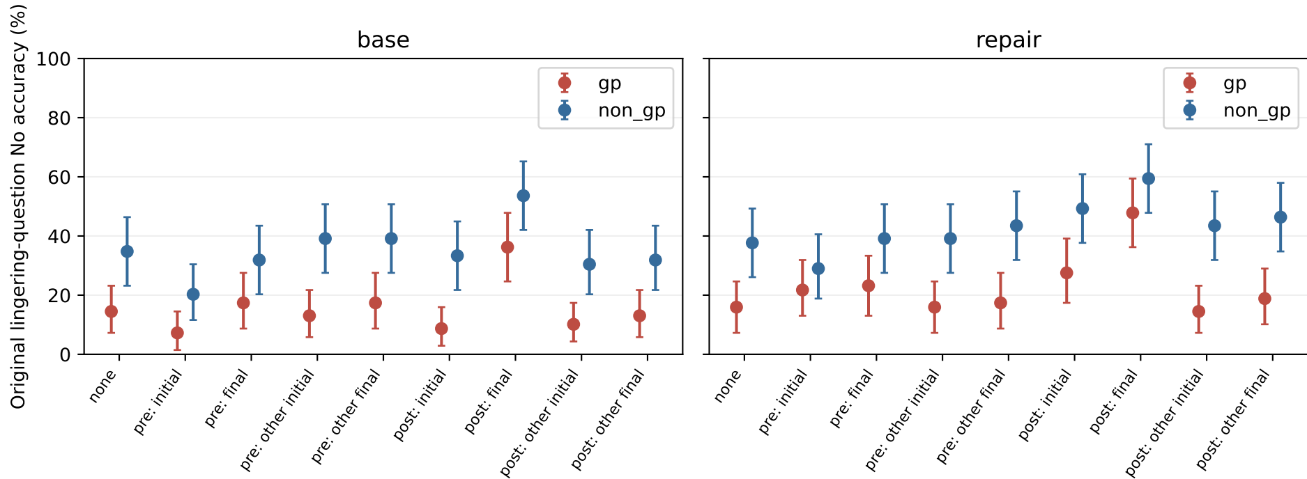
E08: target always follows sentence; 69 paired lexical sets, bootstrap 95% CI
