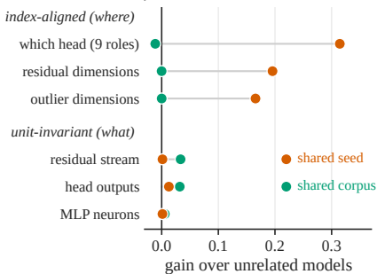
(c) Coordinates inherited, content learned
