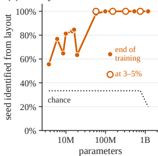
(b) The layout identifies the seed
