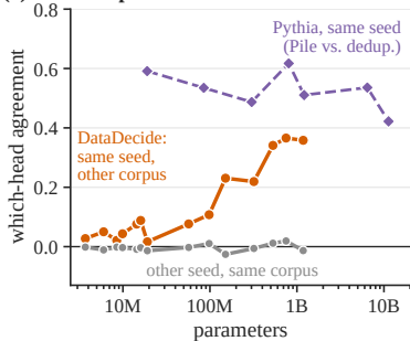
(a) The seed places the heads
