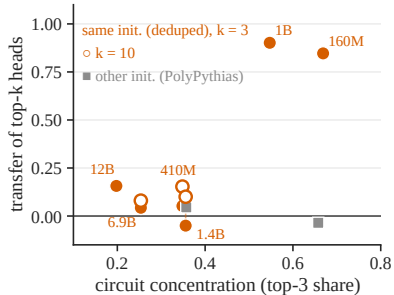
(a) Pythia: IOI, Pile vs. dedup.
