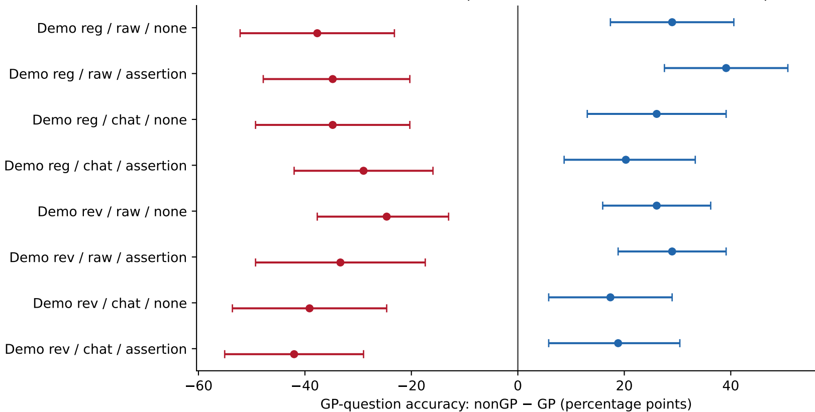
Qwen3-8B: query order reverses the condition effect Fixed demo bundle; full FP32; 69 paired lexical sets; 95% cluster bootstrap CI
