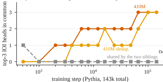
a Pythia-410M siblings: final carriers in place
