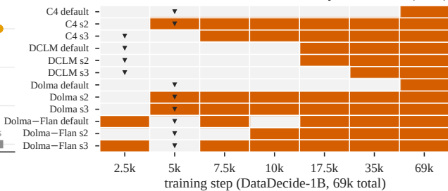
b DataDecide-1B: main carrier is already the final one (filled)
