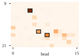
direct effect on IOI
